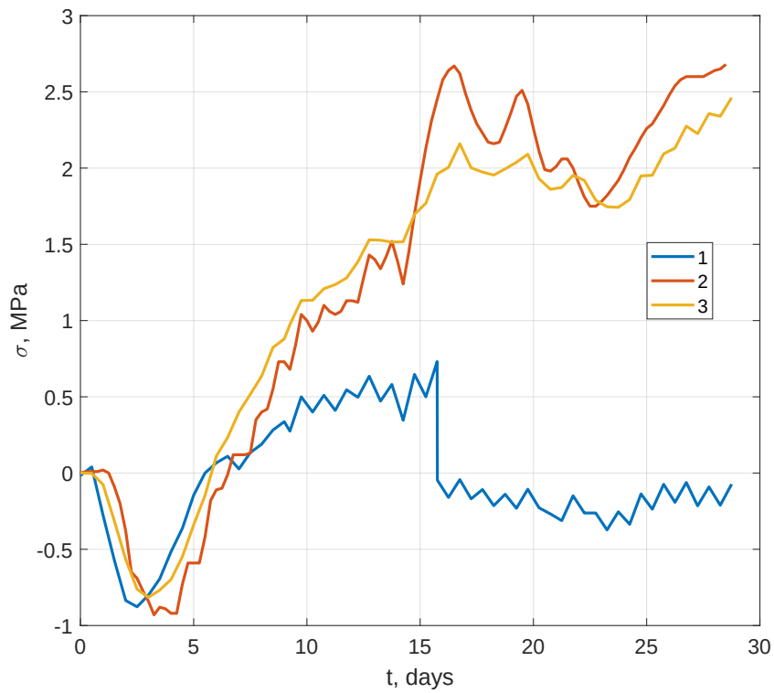
Fig. (8). Comparison of the experimental results (line 1) with the calculation results using the proposed method (line 3) and the calculation results given in (line 2) [25].
