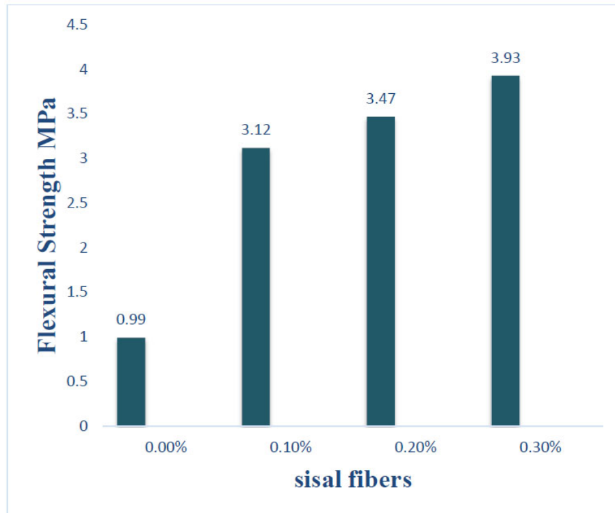
Fig. (7). The relationship between flexural strength and sisal fibers.
