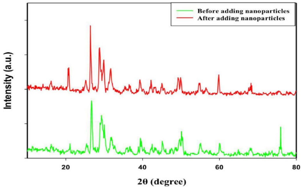
Fig. (13). X-ray diffraction of AAC.
