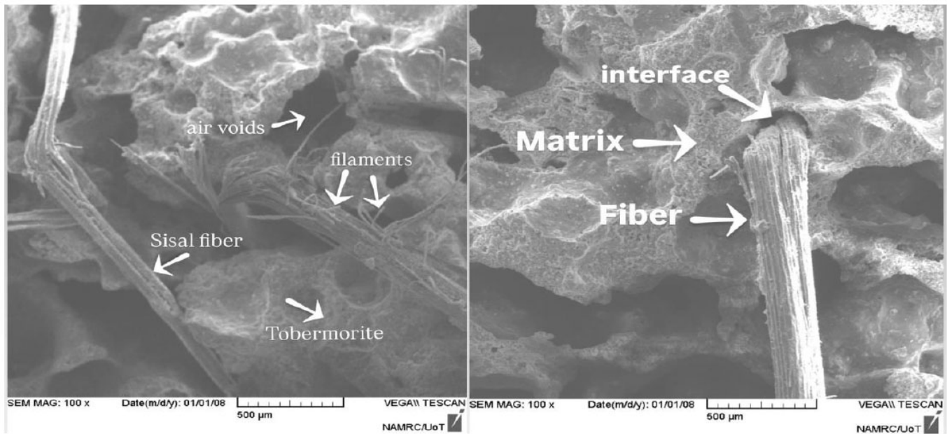
Fig. (12). A scanning electron micrograph (SEM) of autoclaved aerated concrete (AAC) containing nano aluminum with sisal fibers.
